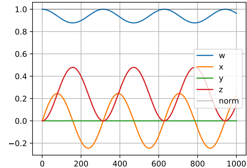
outut quaternon q: (1001, 4)
